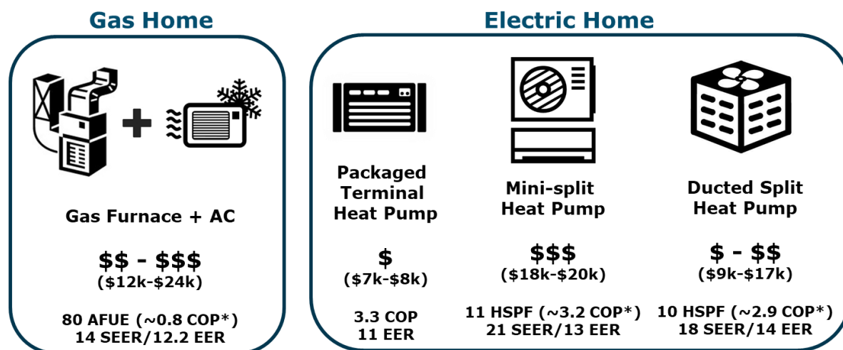
Figure 2-6 Modeled gas and electric HVAC systems: technology, price range and efficiency
