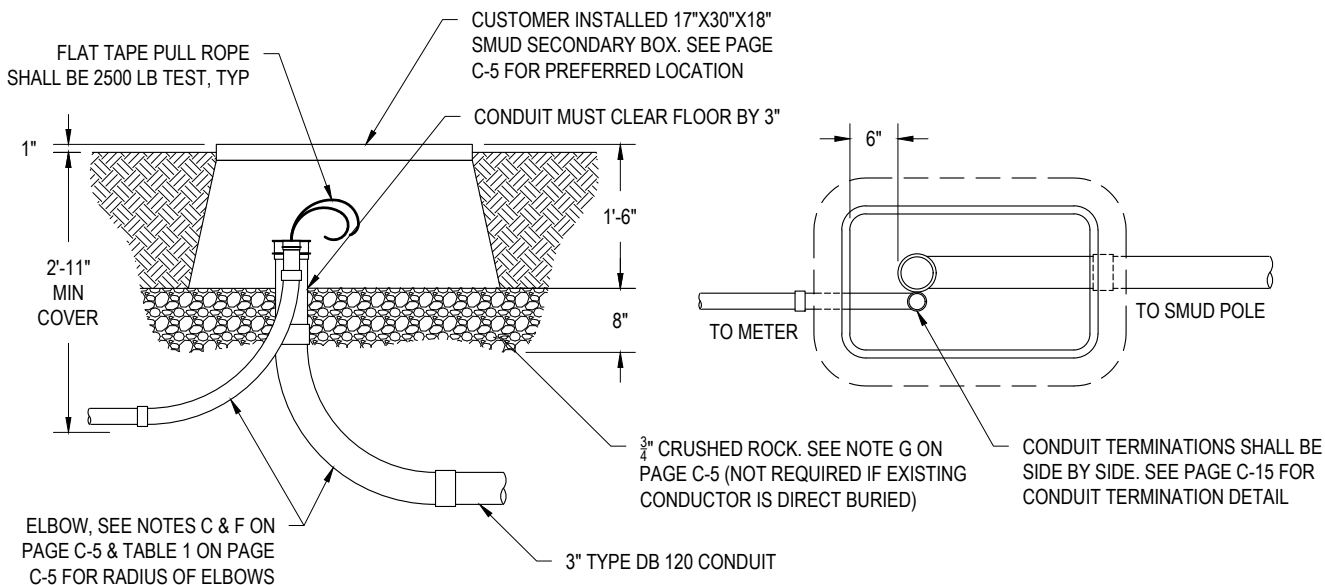
SECONDARY BOX DETAIL
