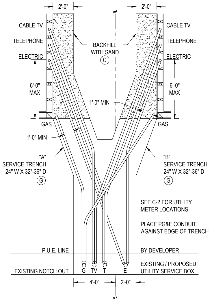
DETAIL - 1 TYPICAL SERVICE CONDUIT RUNS DETAIL
