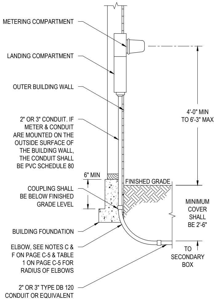
METER DETAIL
