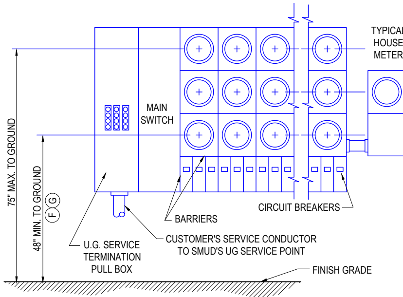
FIGURE 2 TYPICAL MULTI-METER INSTALLATION 7 METERS OR MORE
