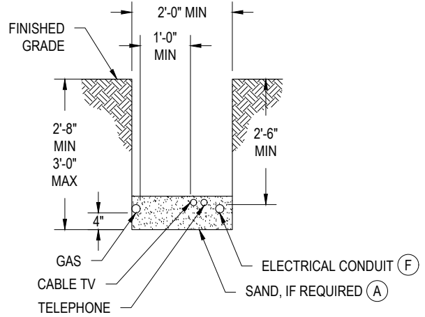
TYPICAL JOINT SERVICE TRENCH DETAIL
