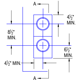
METER SOCKET SPACING DETAIL
