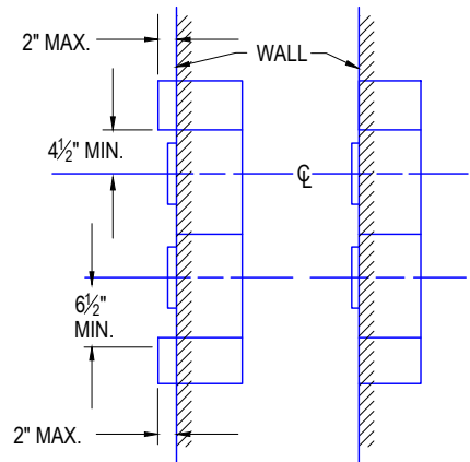
SECTION A-A RECESSED METER SOCKETS
