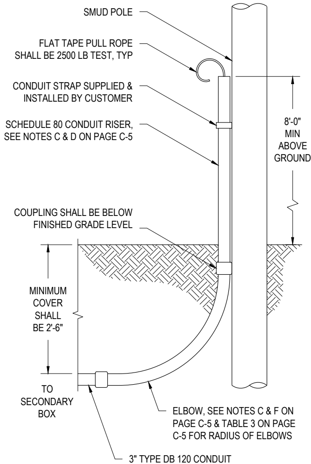
SECONDARY RISER DETAIL
