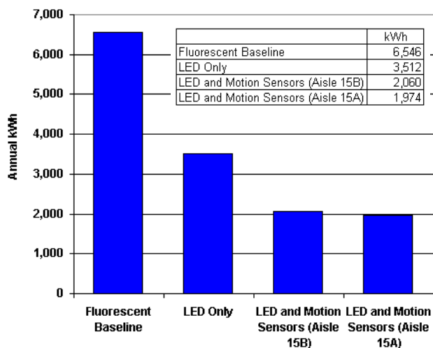
Figure 9: The combination of LEDs and motion sensors reduced energy consumption by over 68% for the cases with the prototype sensors (Aisle 15A) as well as the production sensors (Aisle 15B). Each aisle has three 5-door freezer cases.
